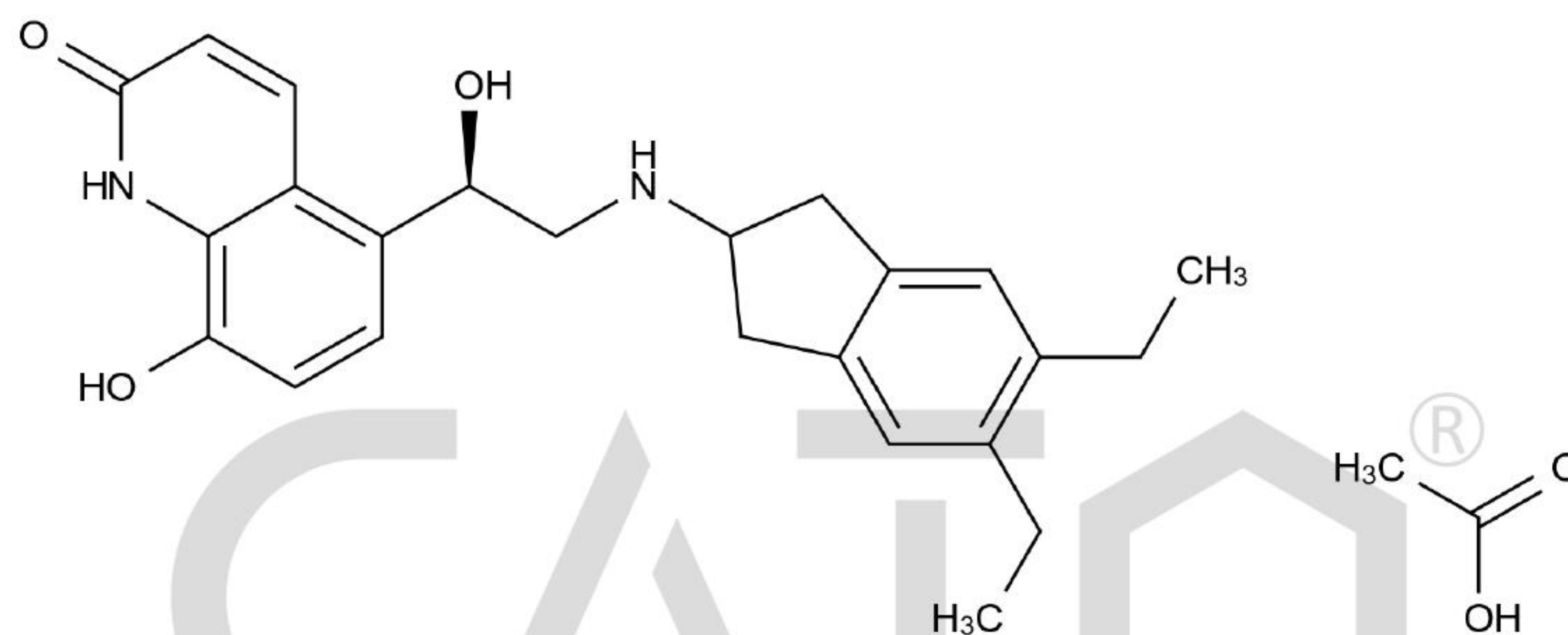
Chemical Structure:
