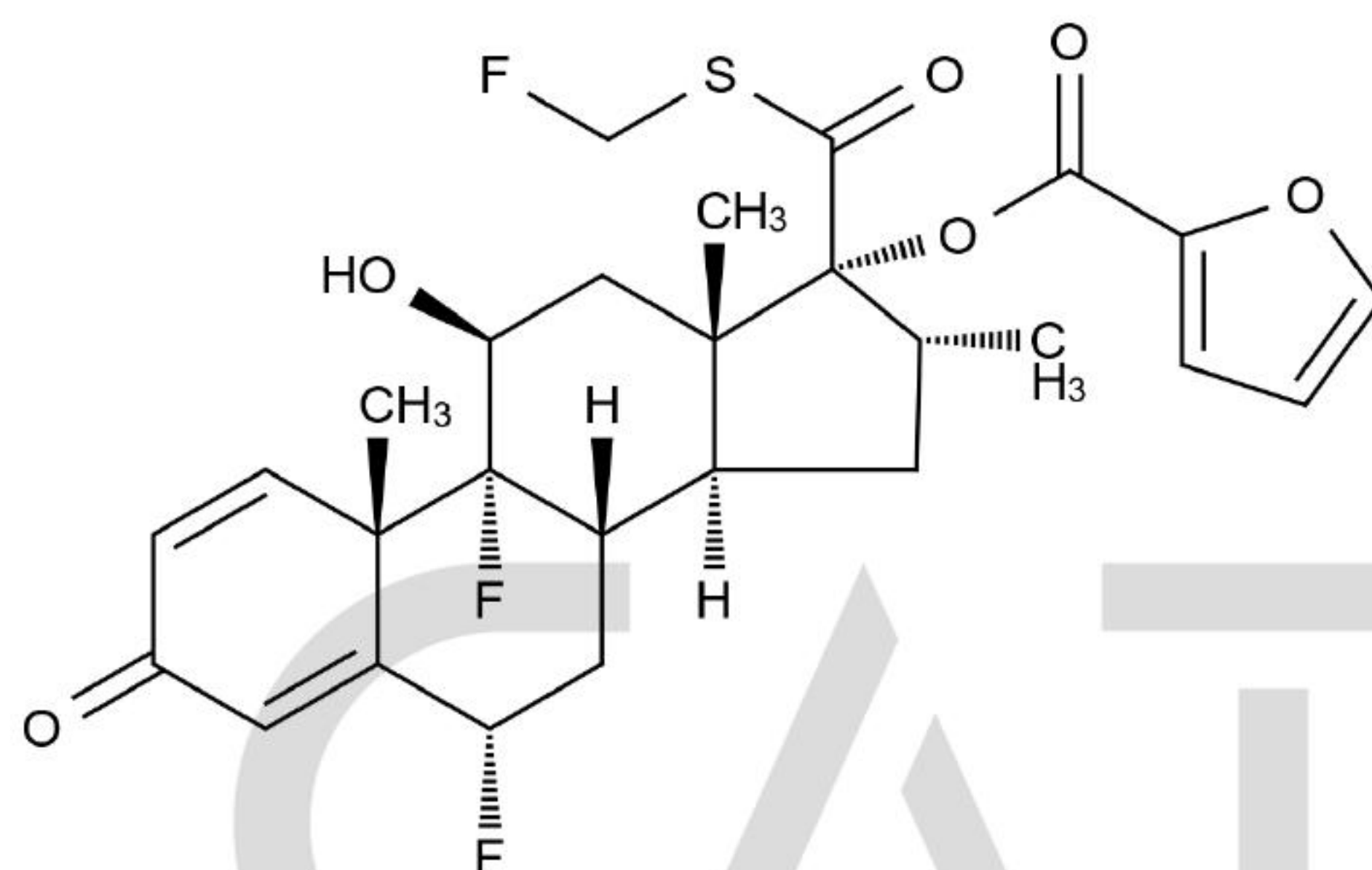
Chemical Structure:
