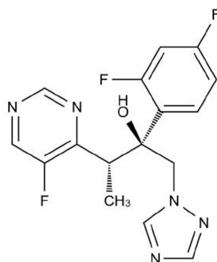
Chemical Structure:
