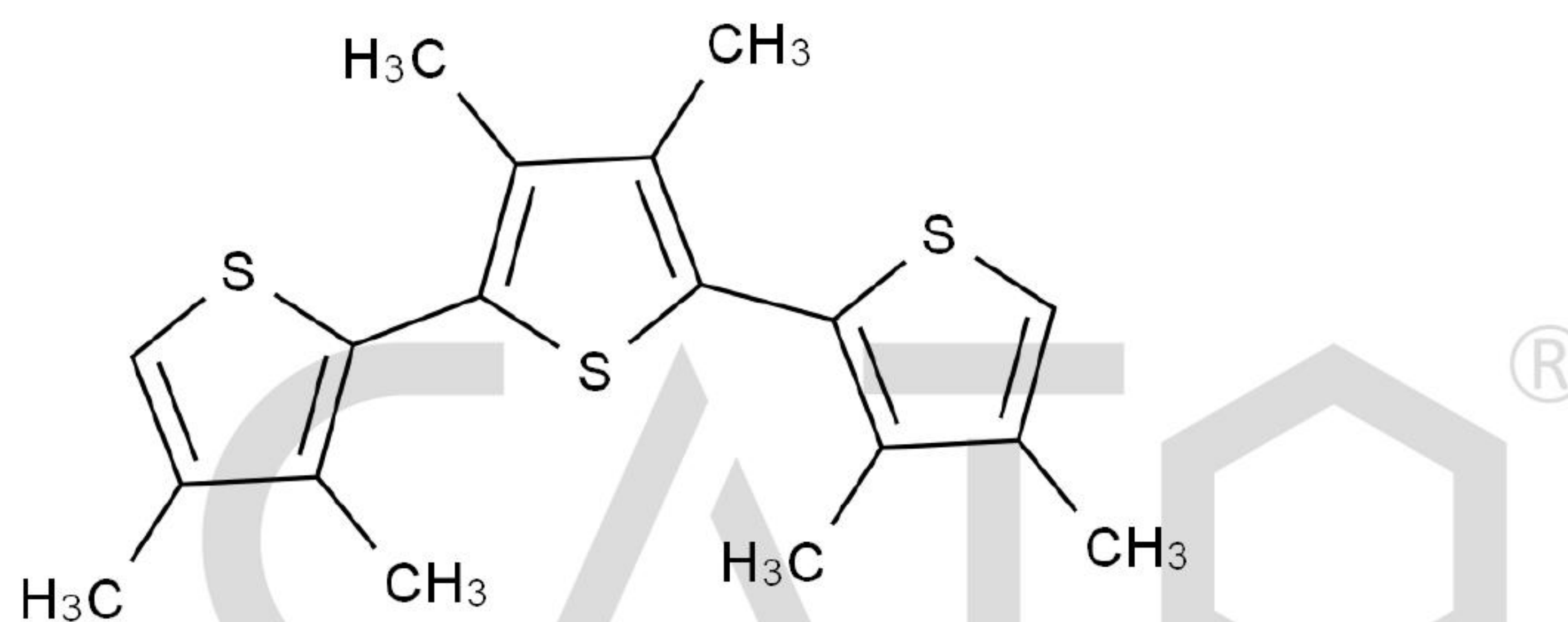
Chemical Structure:
