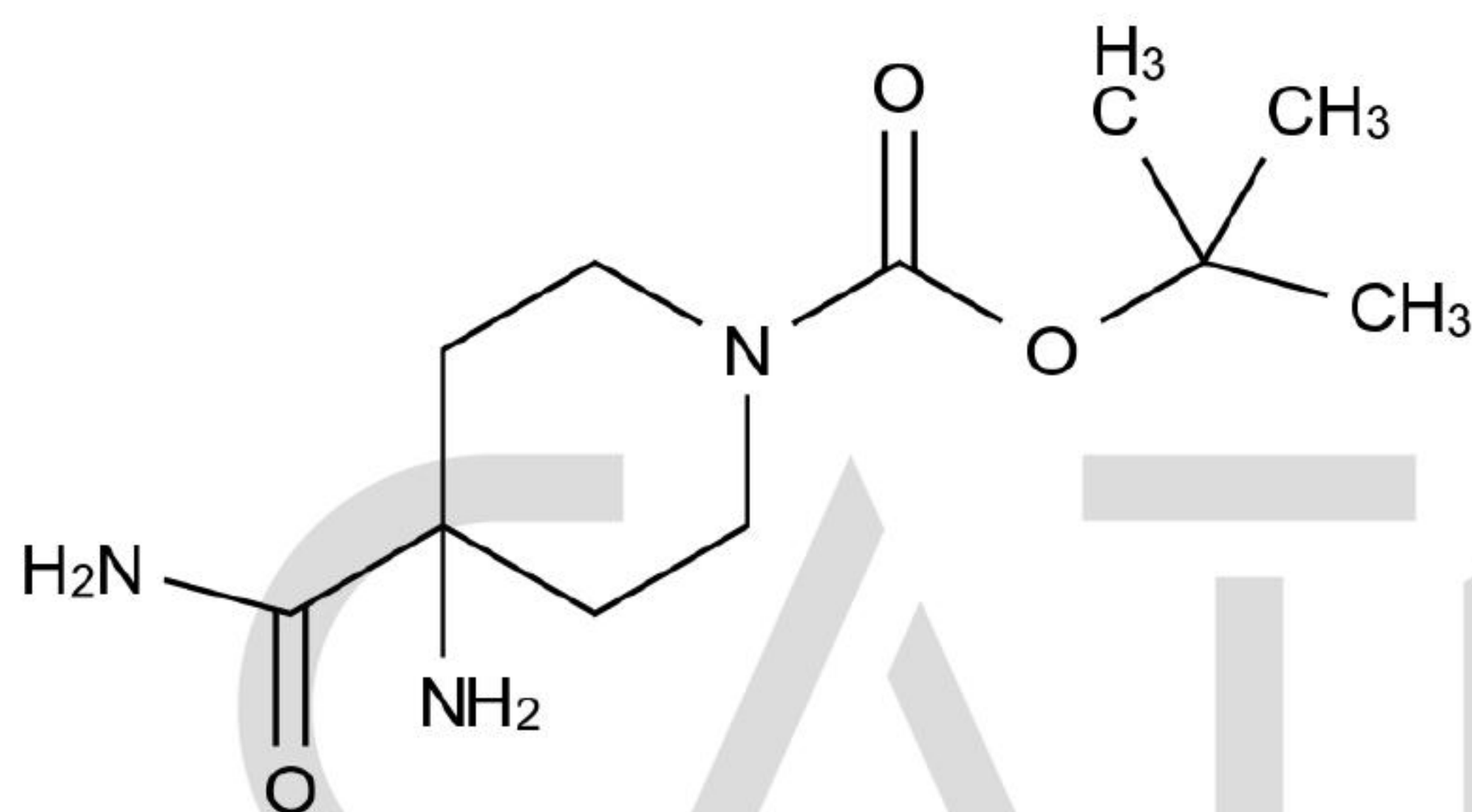
Chemical Structure:
