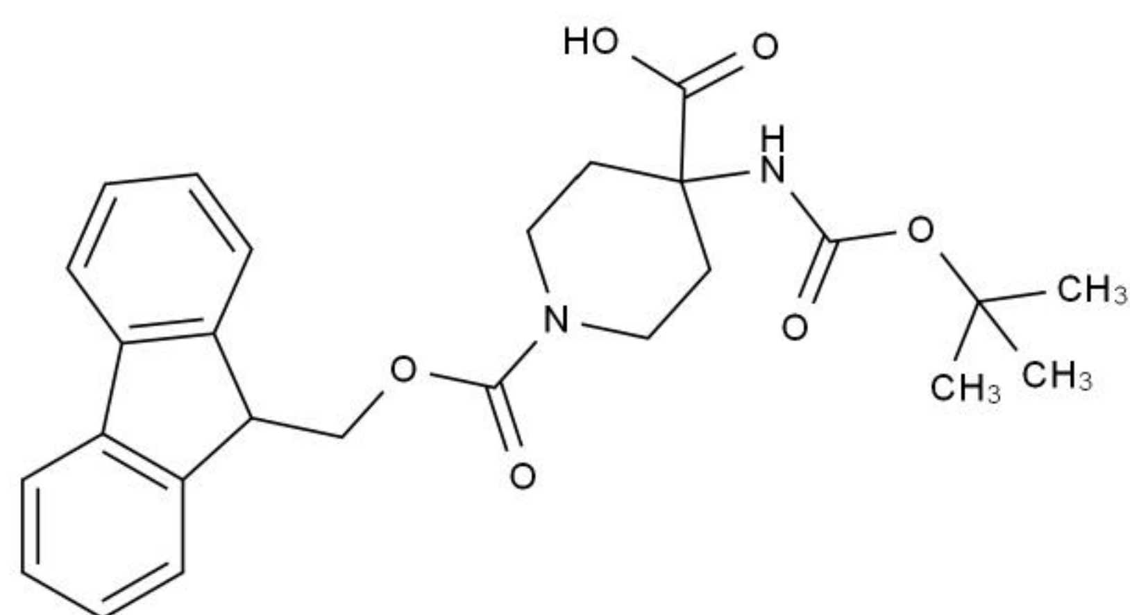
Chemical Structure:
