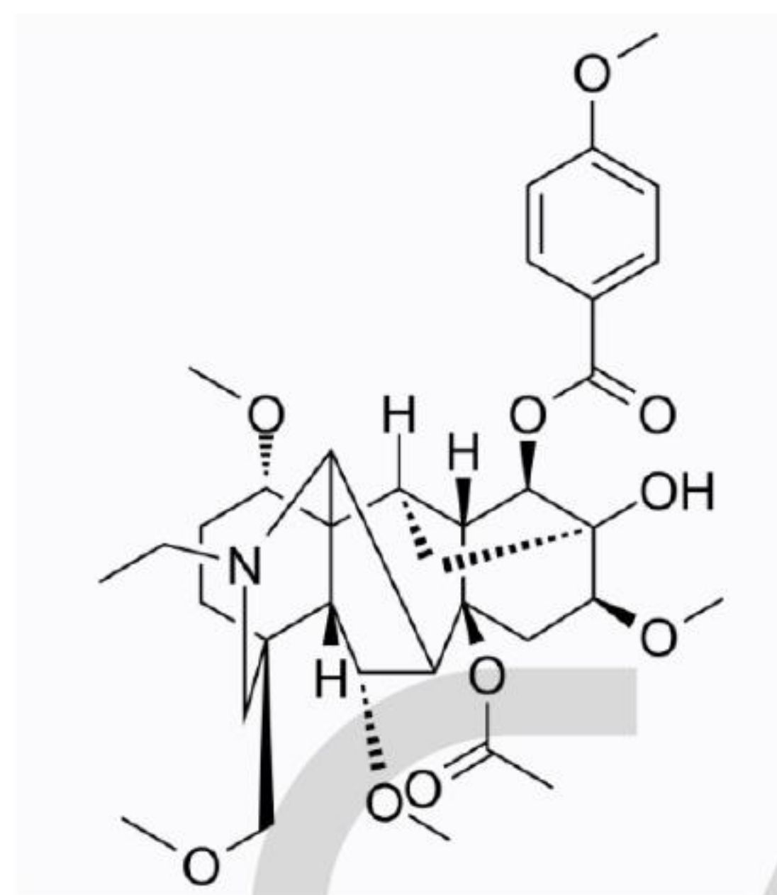
Chemical Structure:
