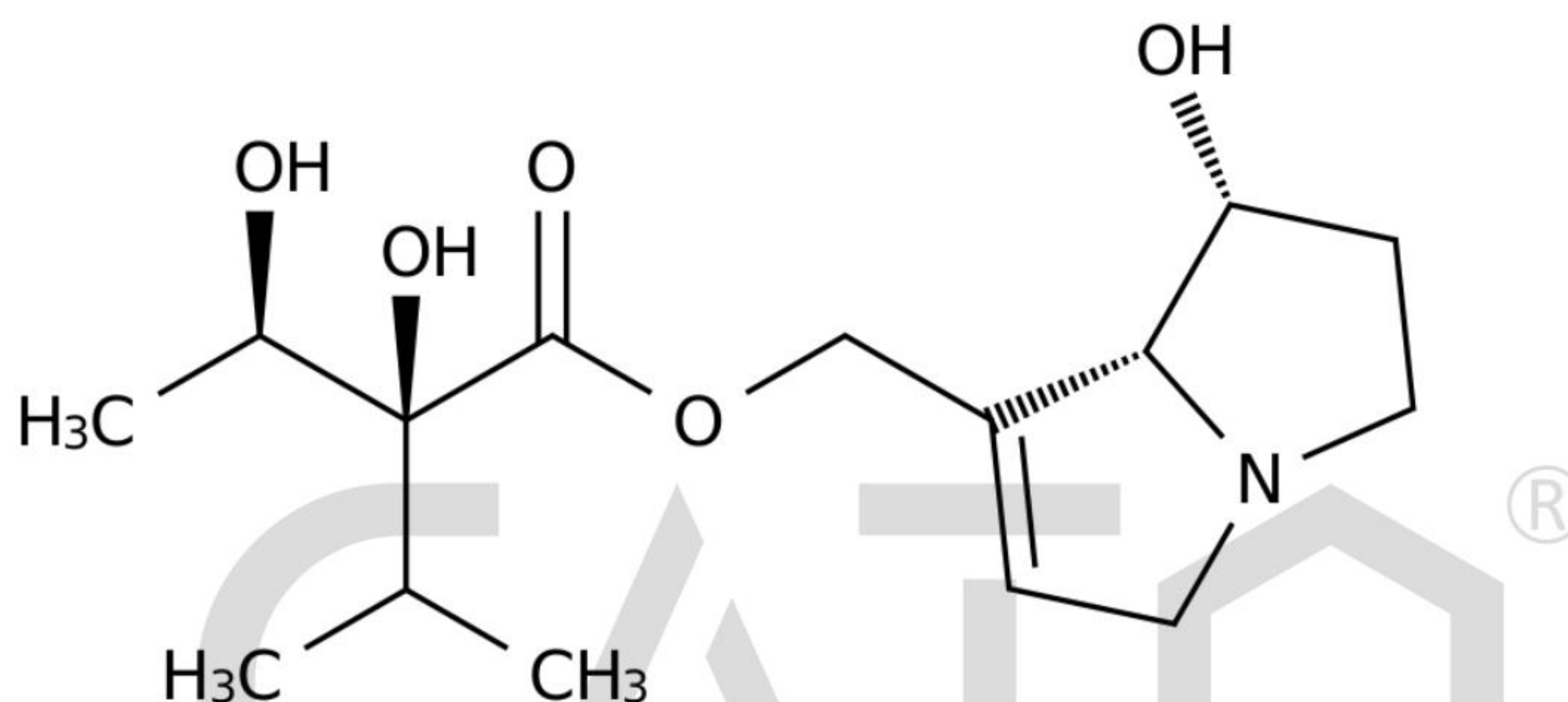
Chemical Structure:
