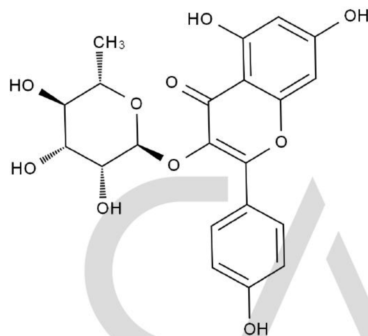
Chemical Structure:
