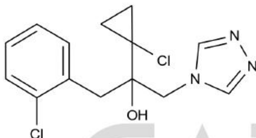
Chemical Structure:
