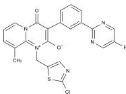
Chemical Structure:
