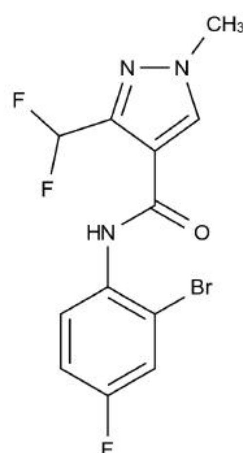
Chemical Structure:
