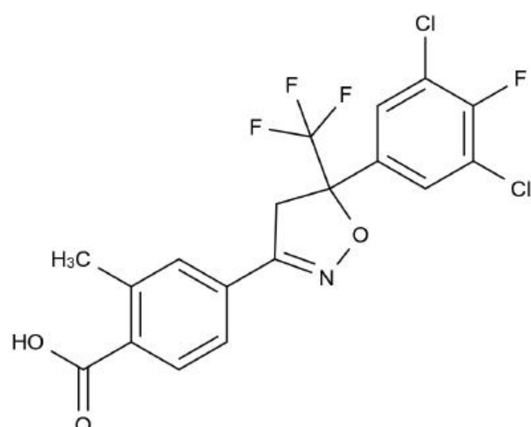
Chemical Structure:
