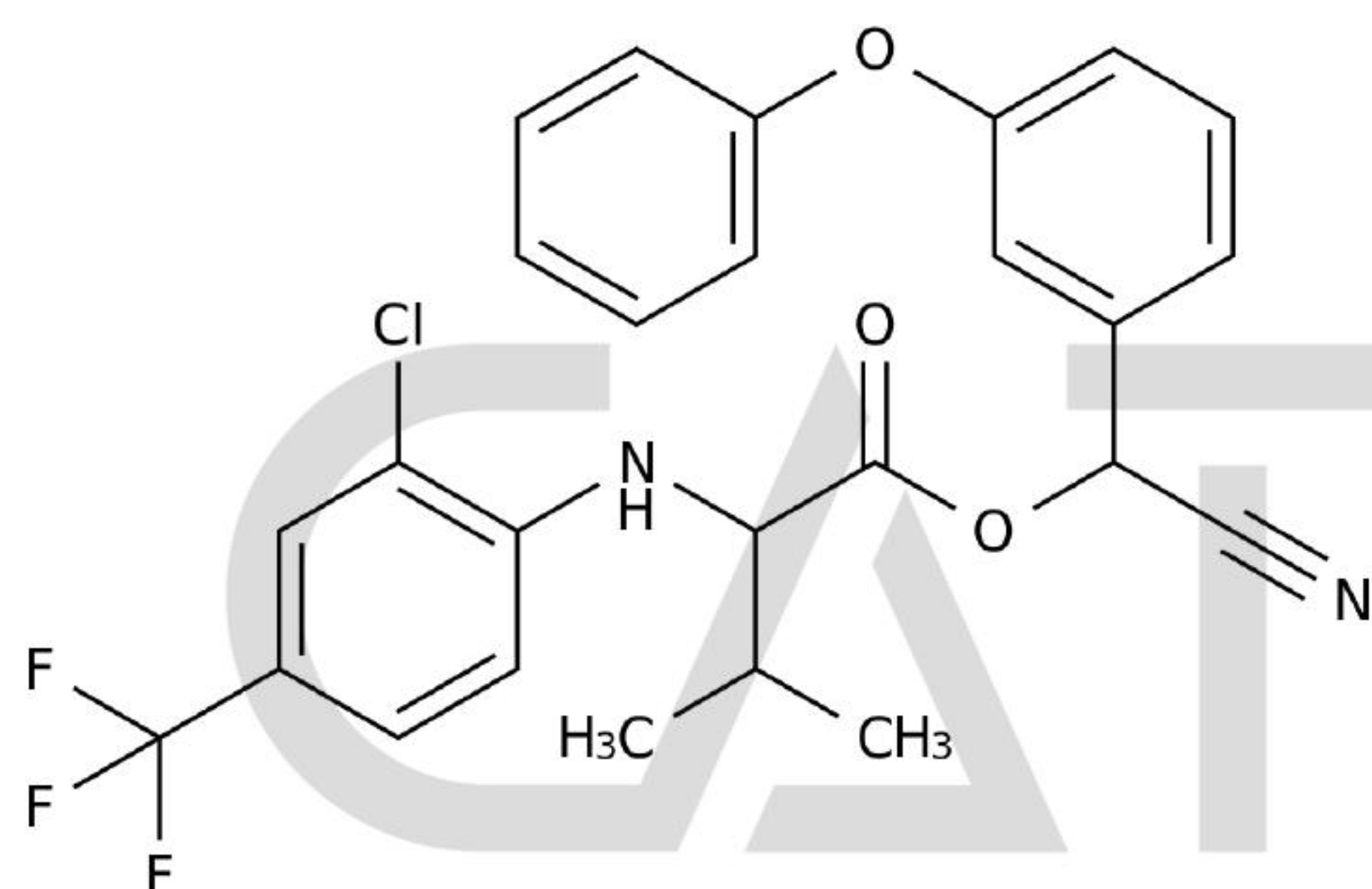
Chemical Structure:
