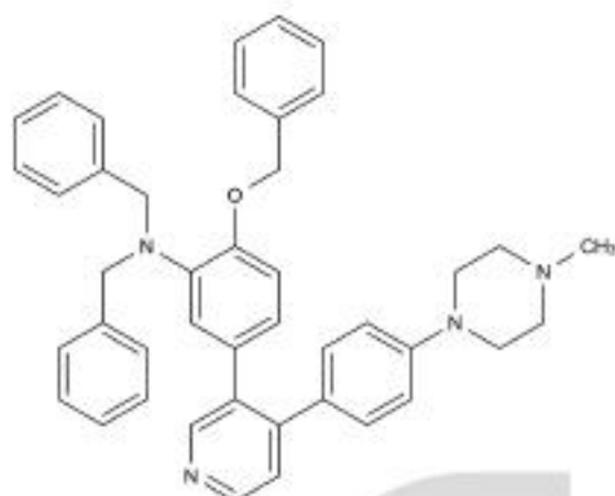
Chemical Structure:
