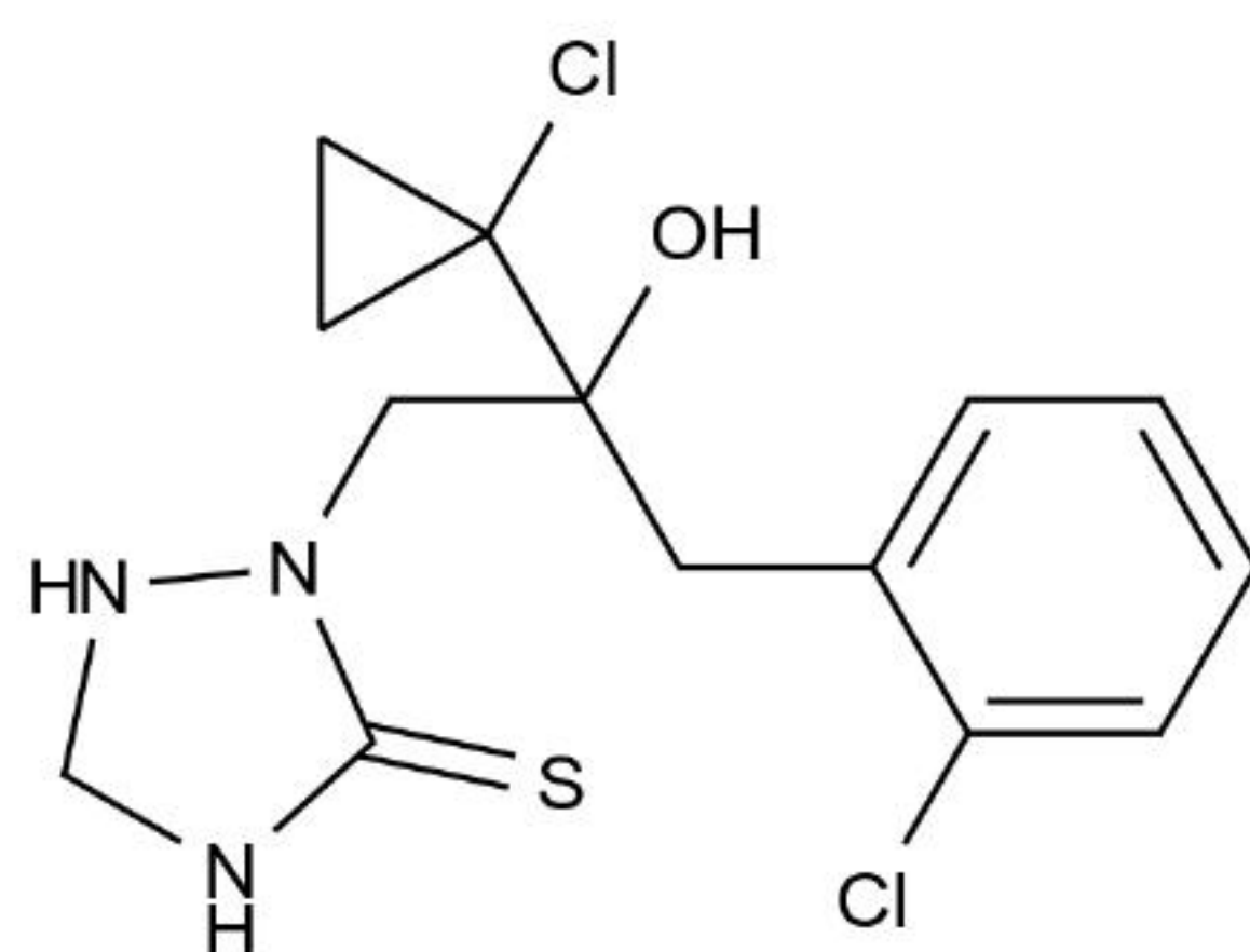
Chemical Structure:
