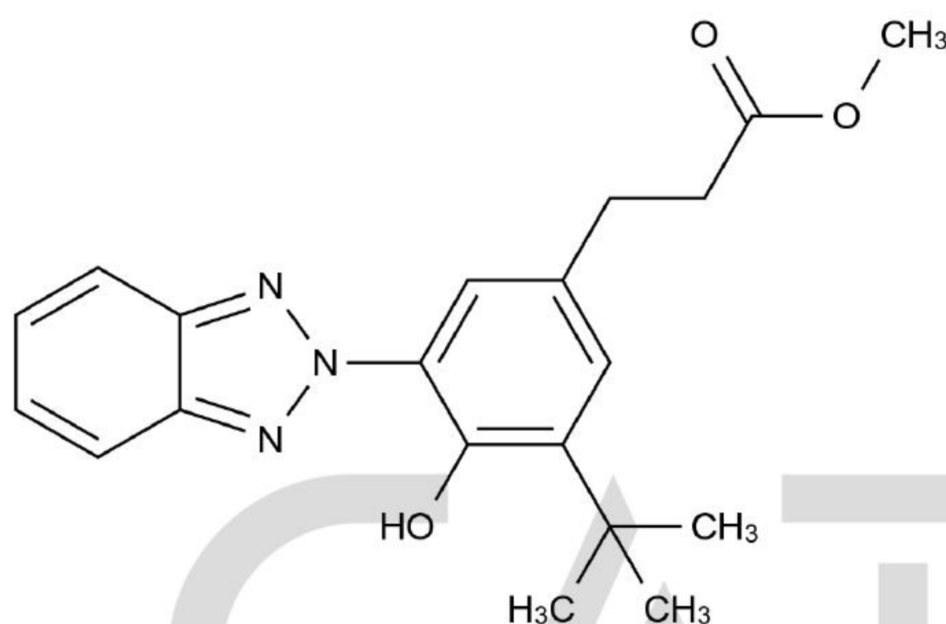
Chemical Structure:
