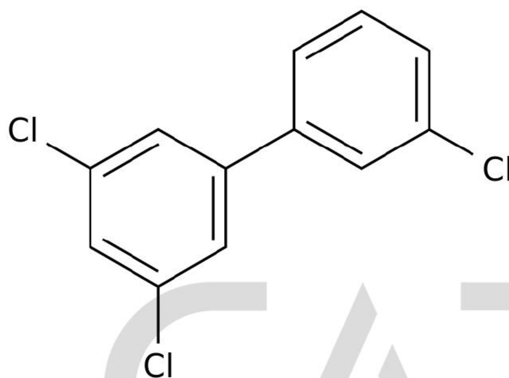
Chemical Structure:
