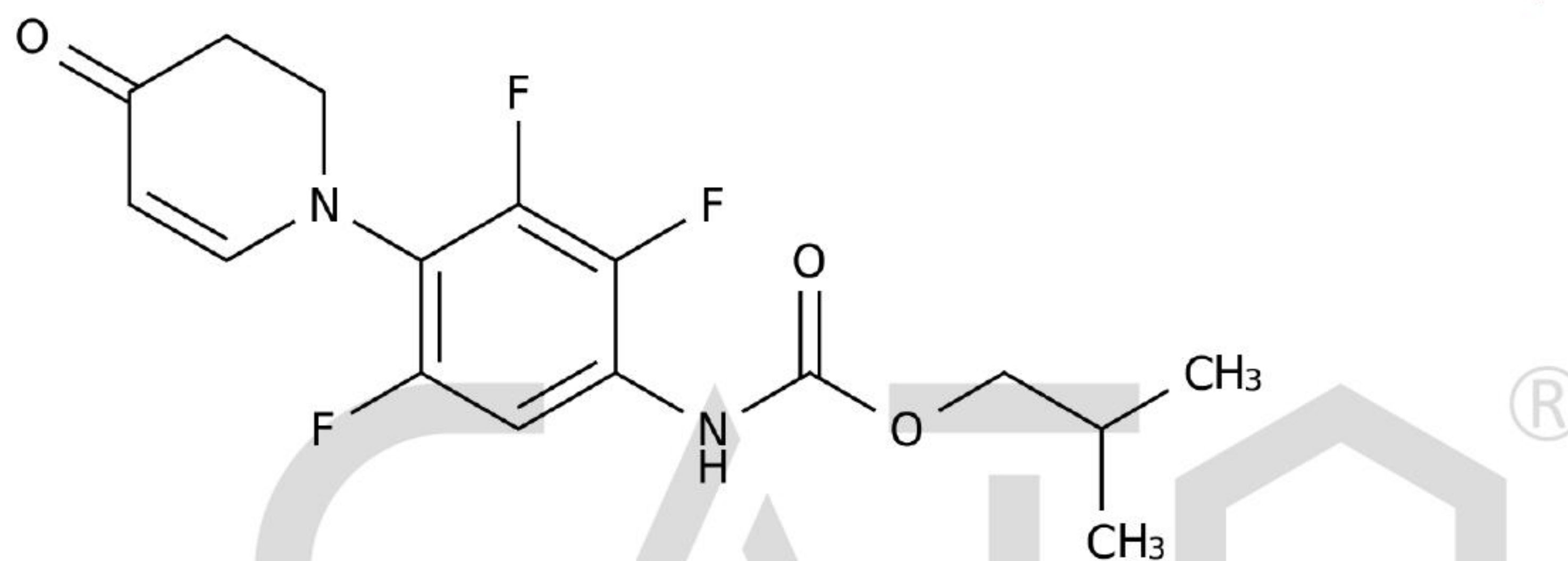
Chemical Structure:
