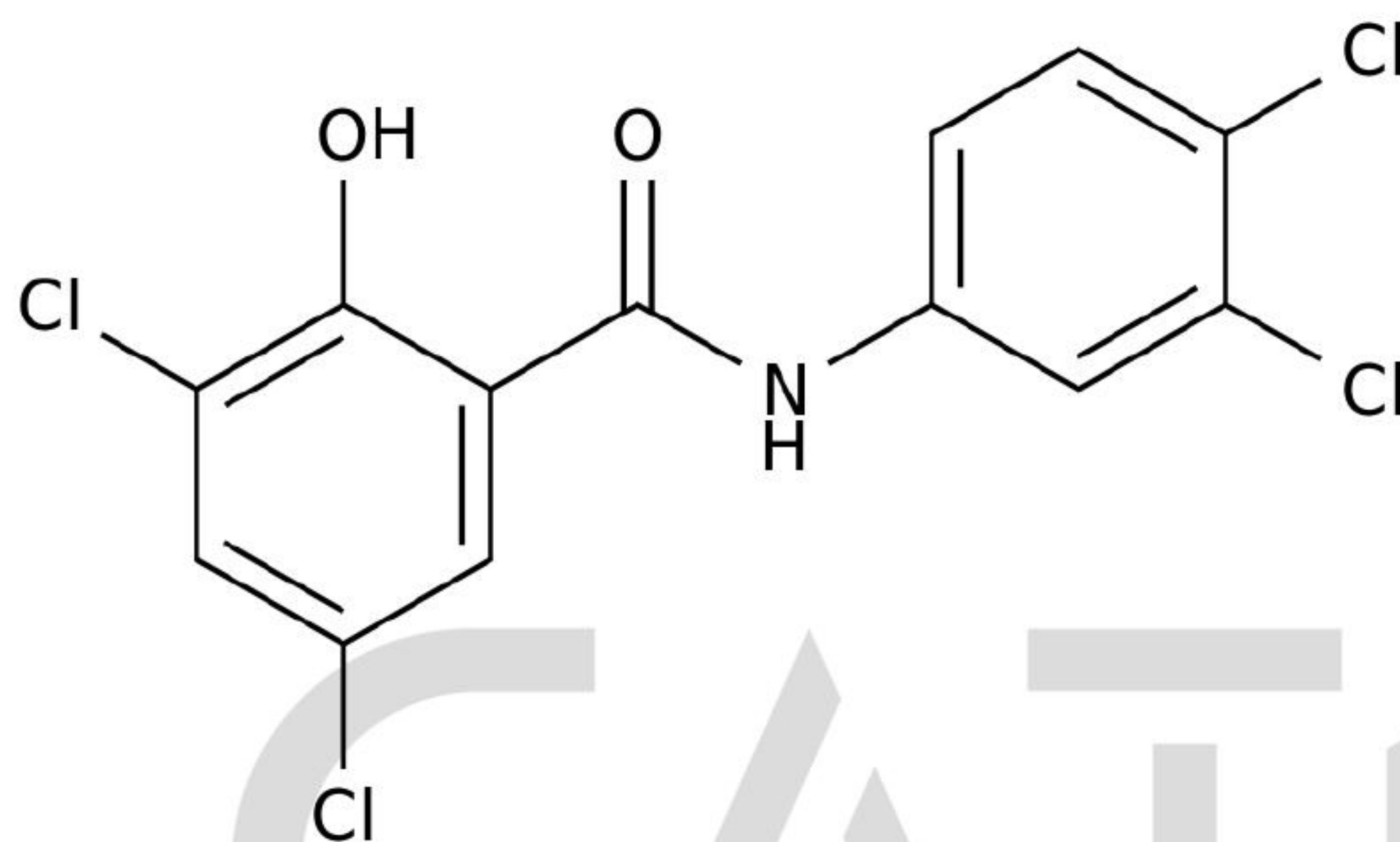
Chemical Structure:
