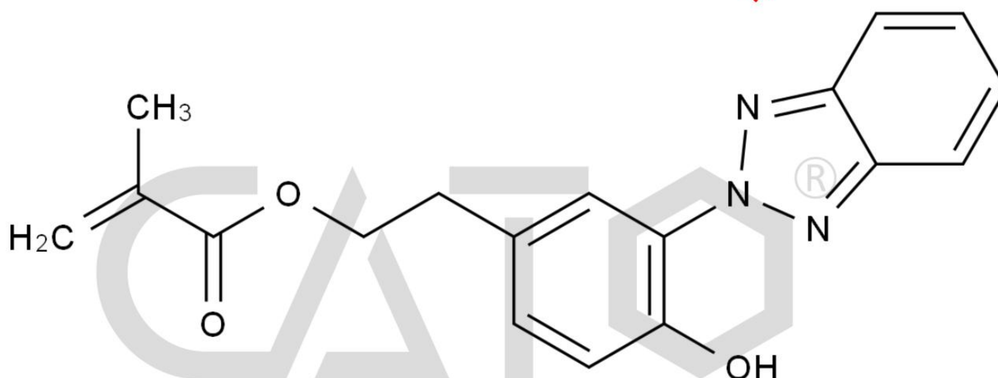
Chemical Structure:
