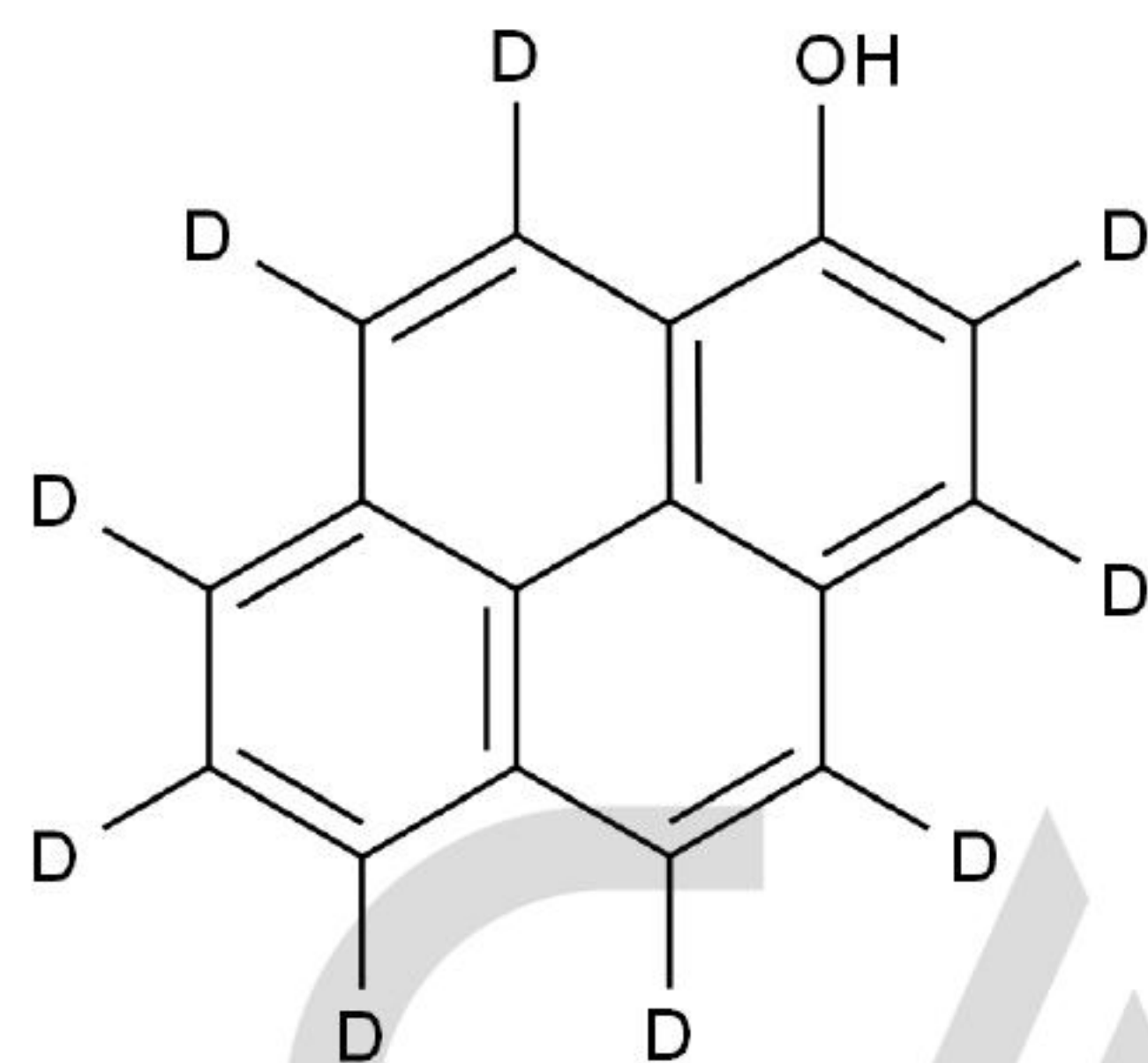
Chemical Structure:
