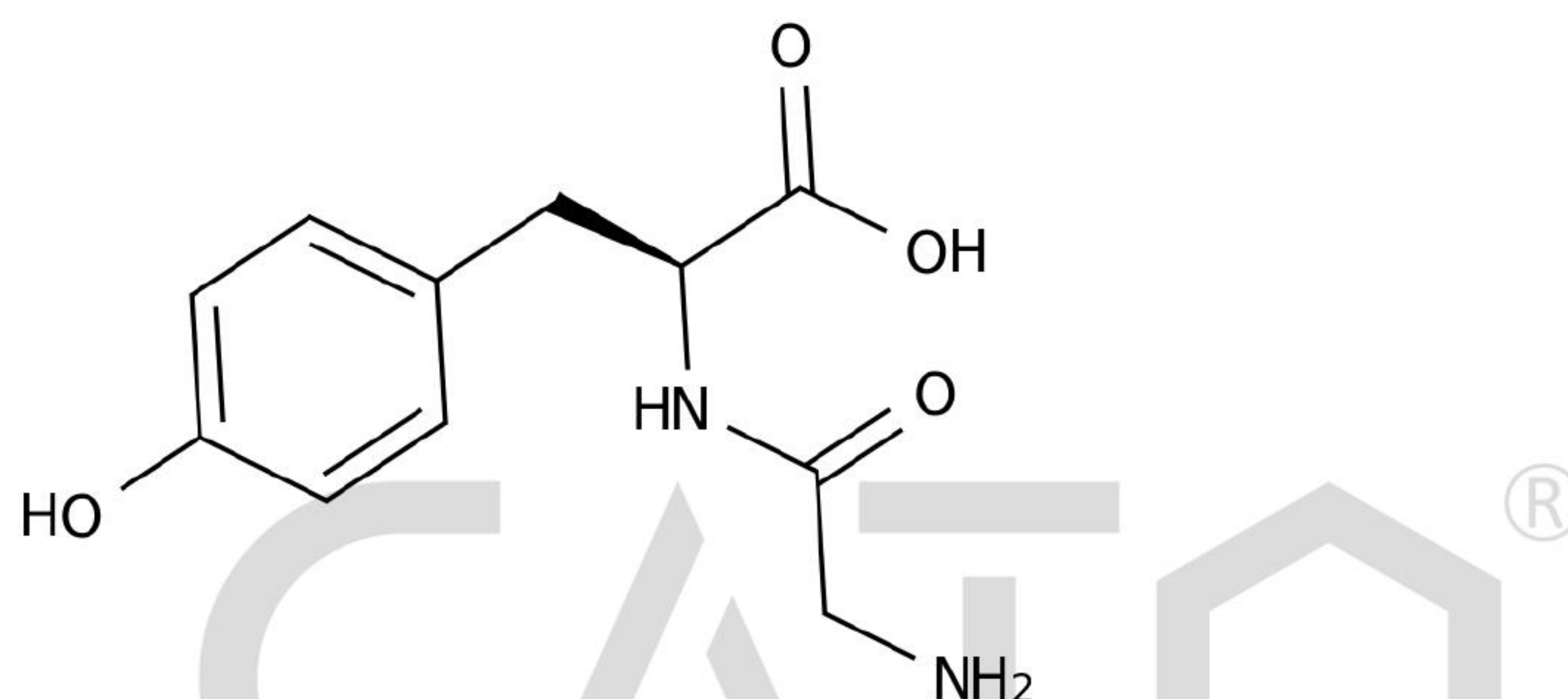
Chemical Structure:
