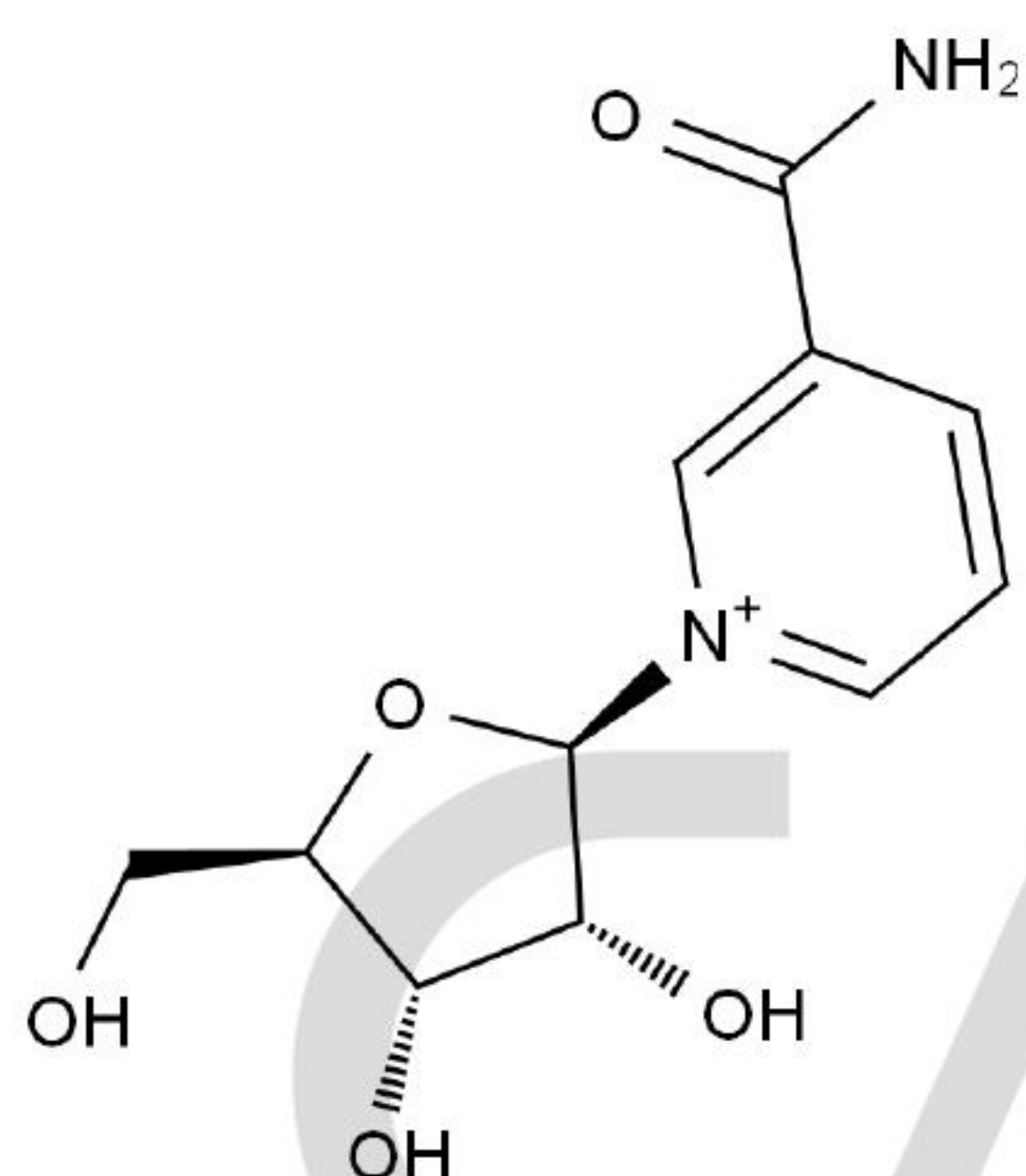
Chemical Structure:
