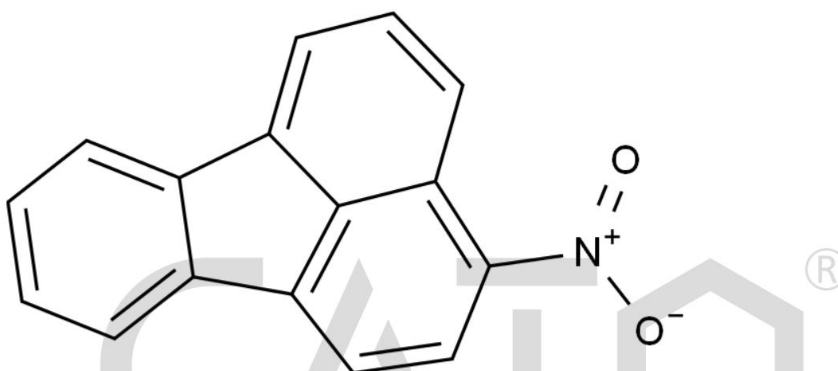
Chemical Structure:
