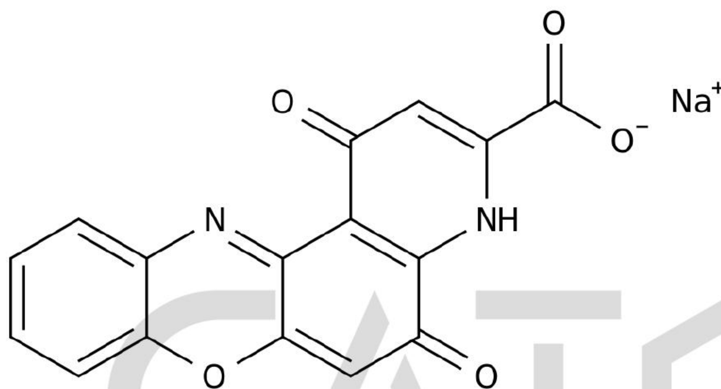
Chemical Structure:
