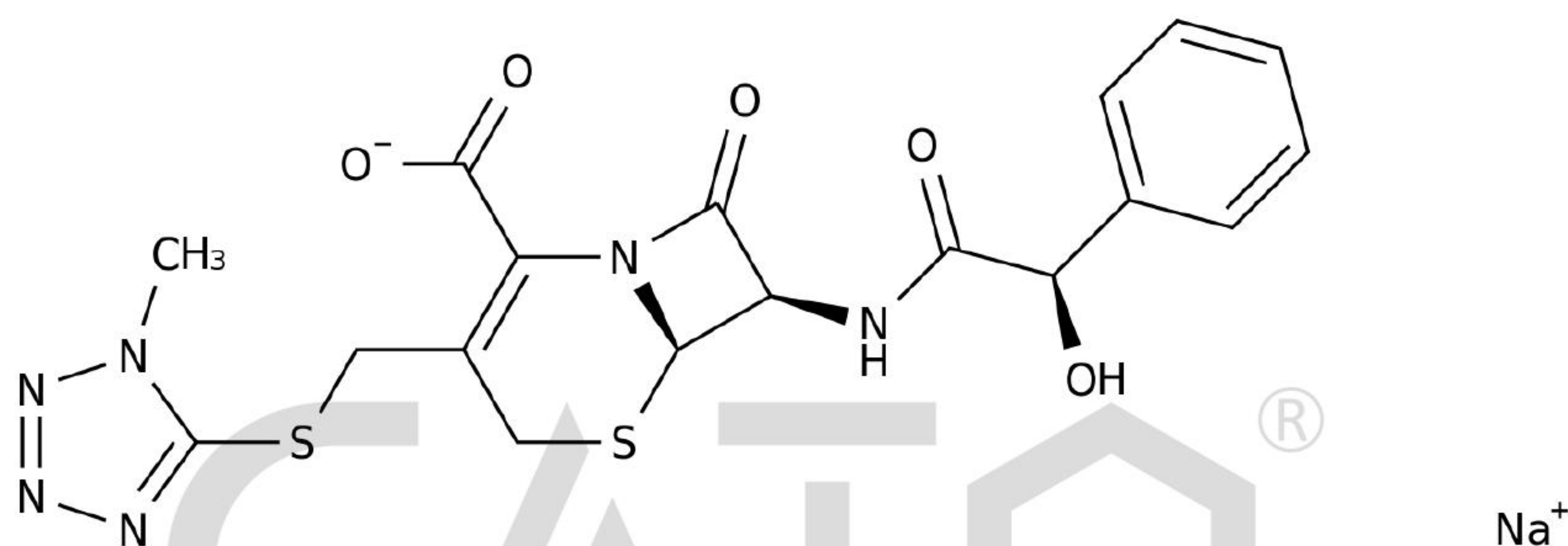
Chemical Structure:
