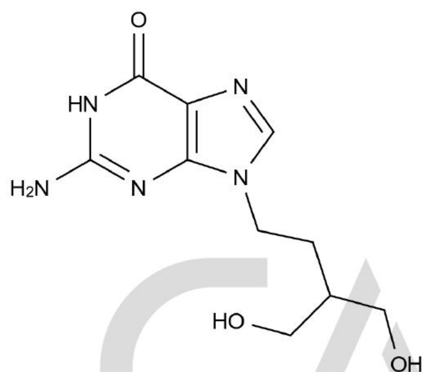
Chemical Structure:
