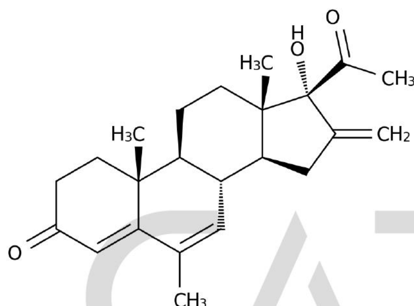
Chemical Structure:
