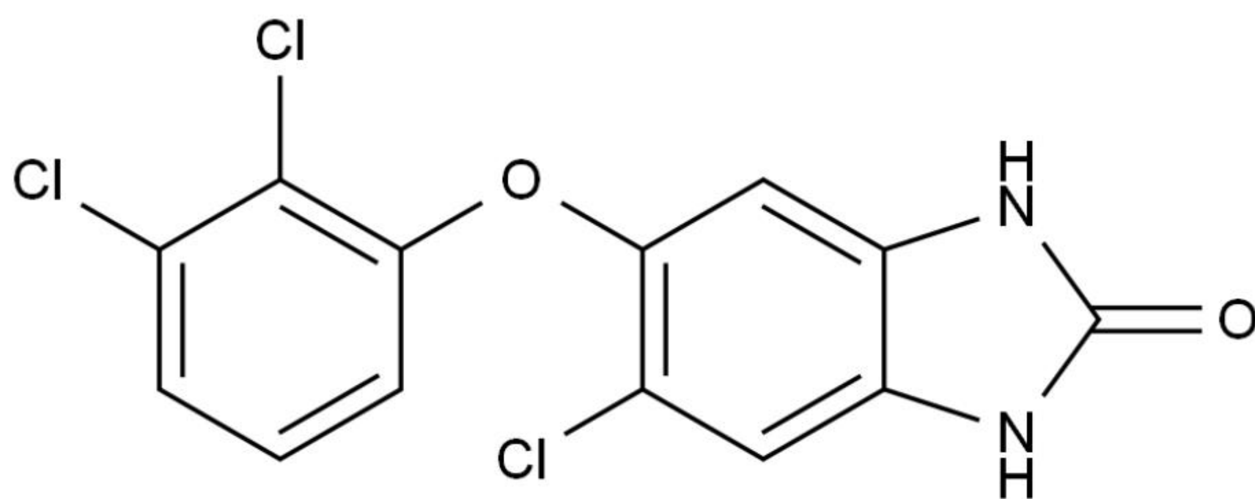
Chemical Structure:
