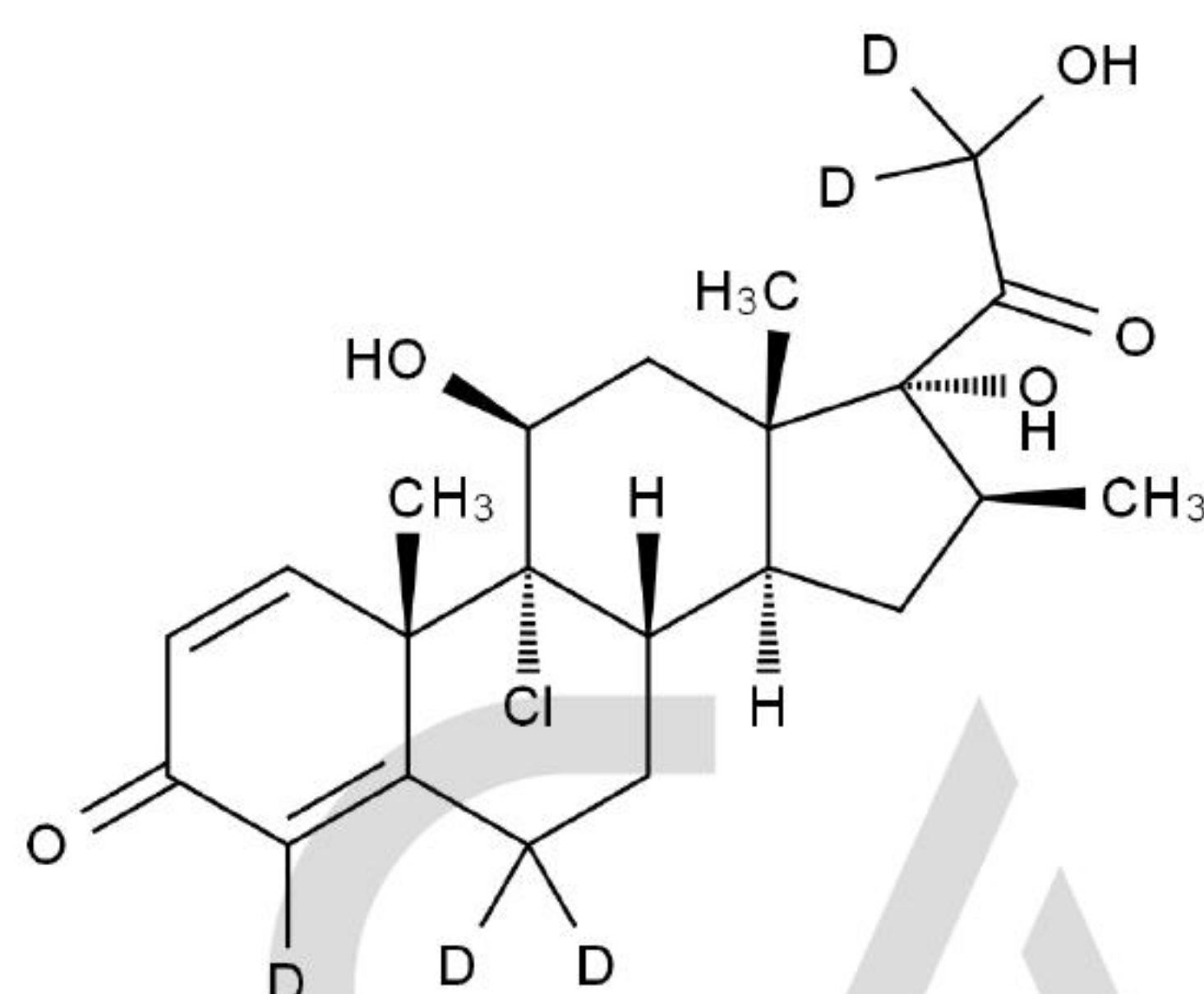
Chemical Structure:
