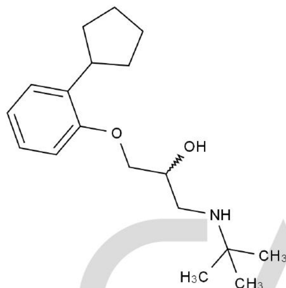
Chemical Structure:
