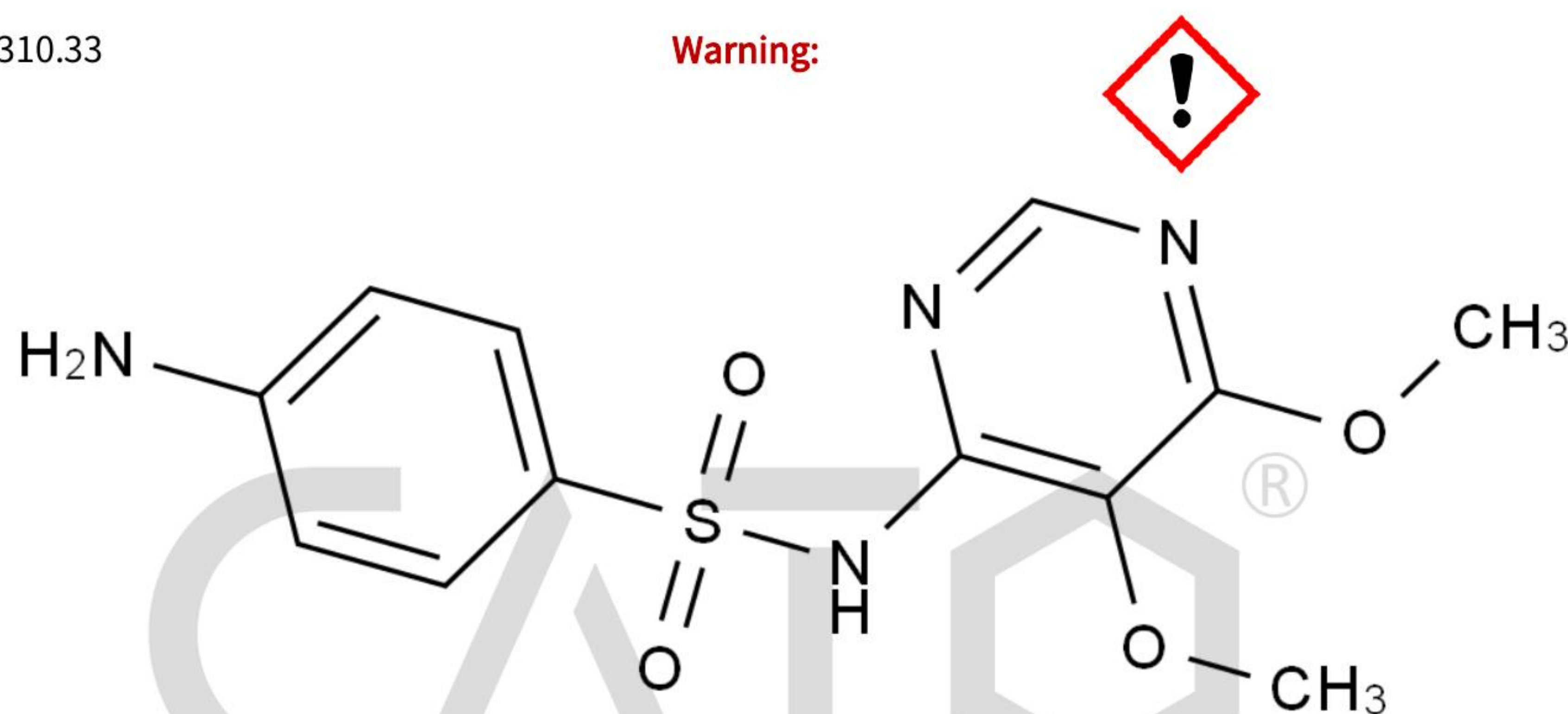
Chemical Structure:
