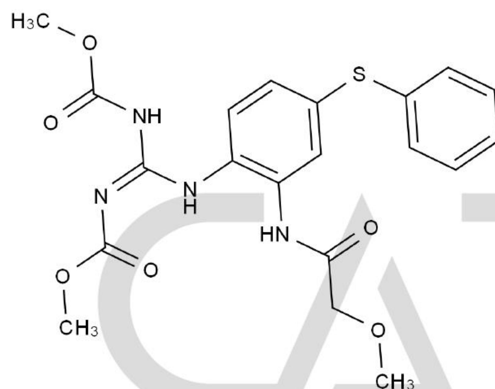
Chemical Structure:
