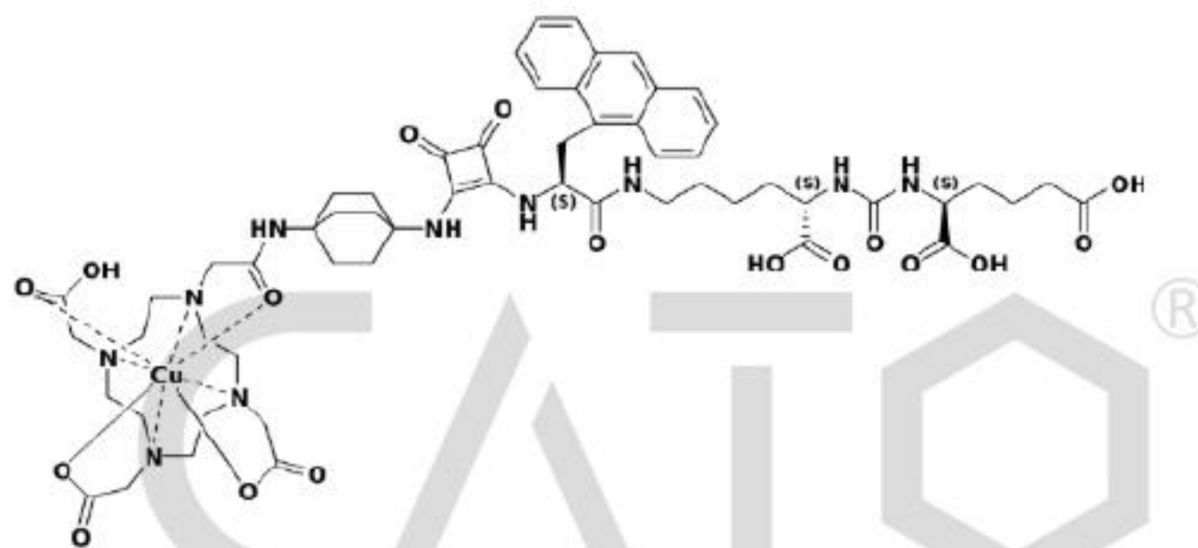
Chemical Structure:
