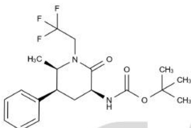
Chemical Structure:
