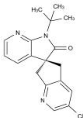
Chemical Structure:
