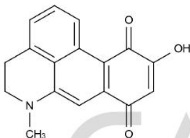
Chemical Structure:
