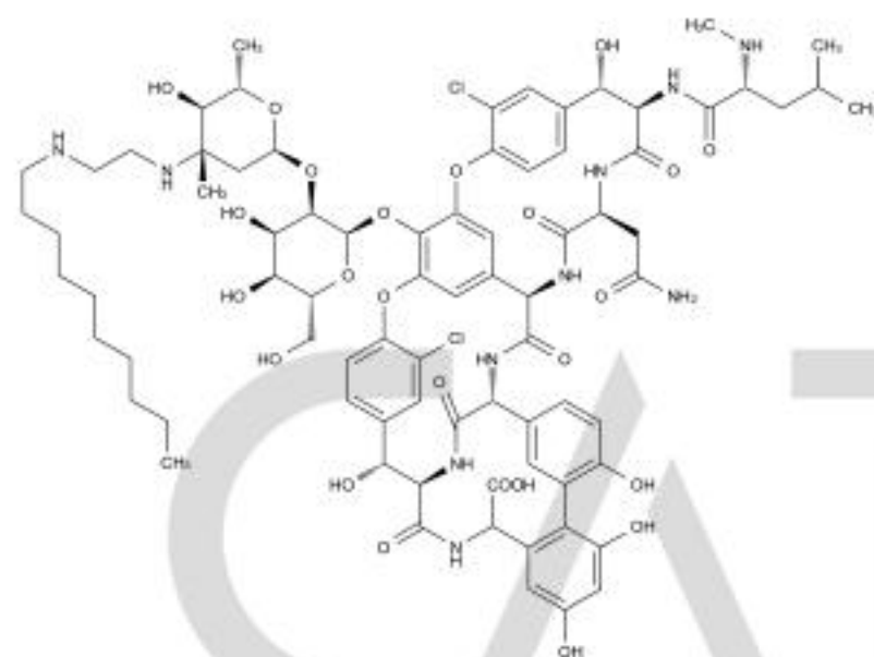
Chemical Structure:
