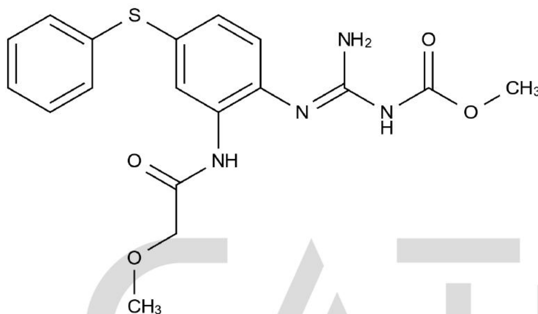
Chemical Structure:
