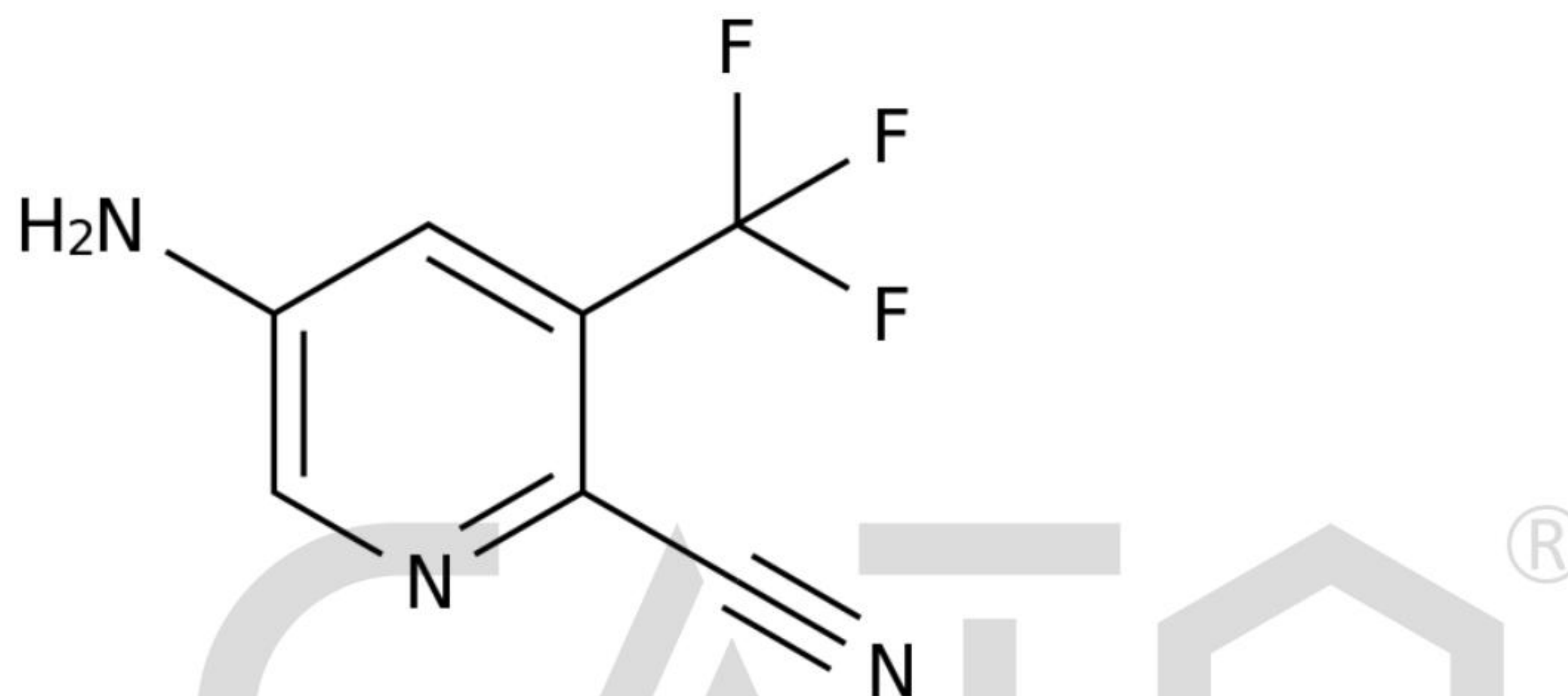
Chemical Structure:
