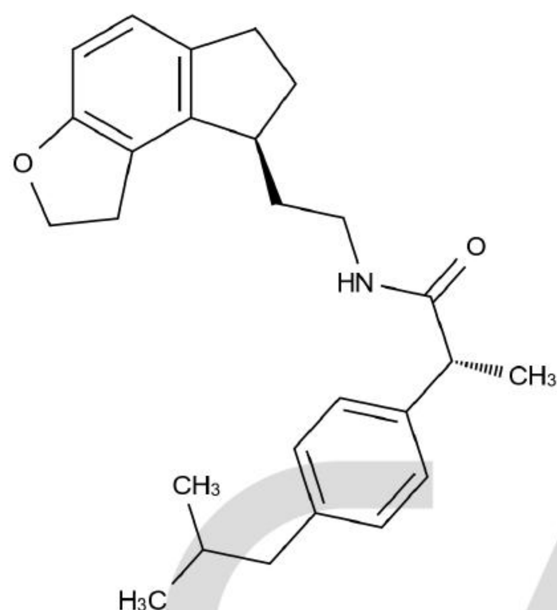
Chemical Structure:
