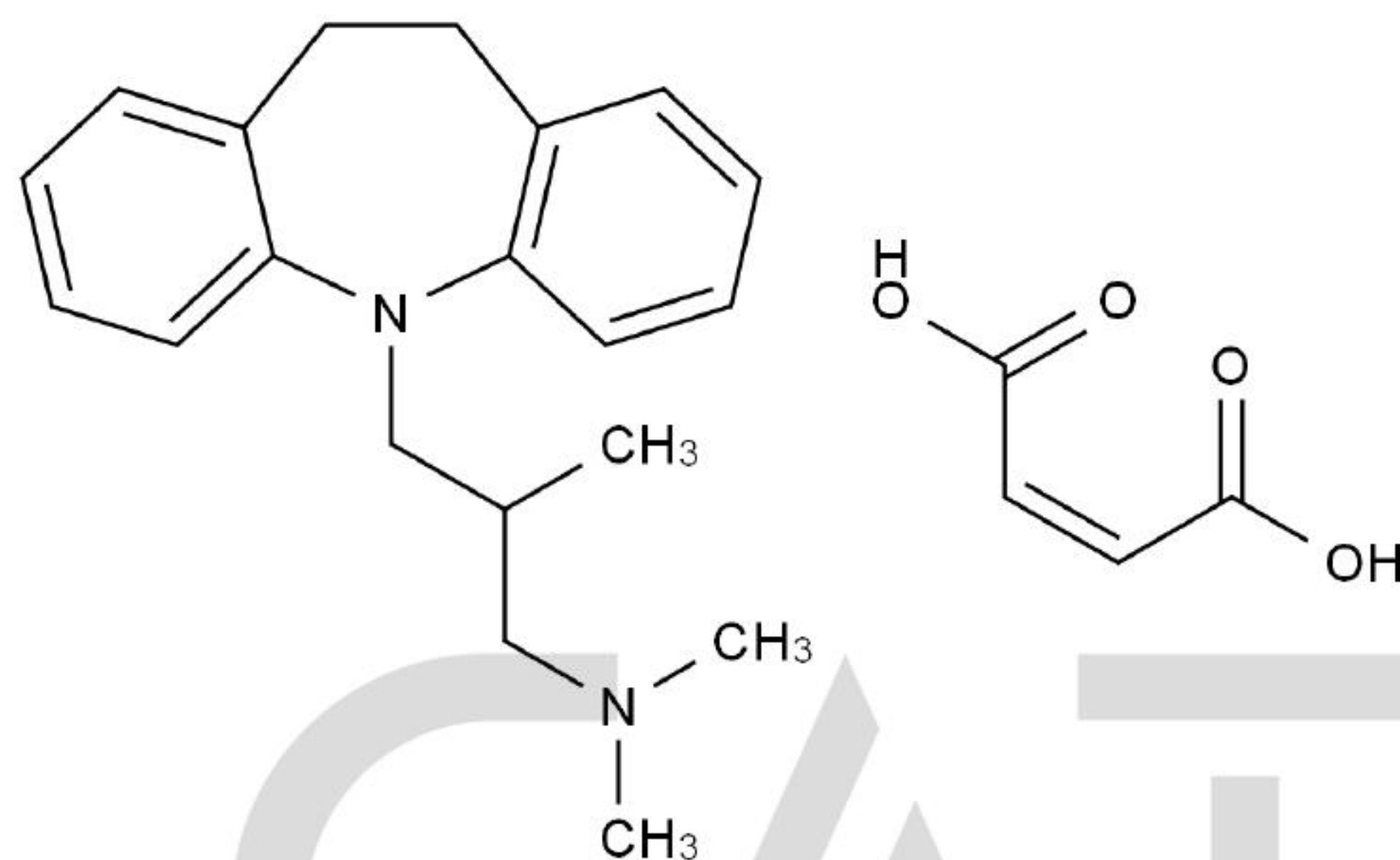
Chemical Structure:
