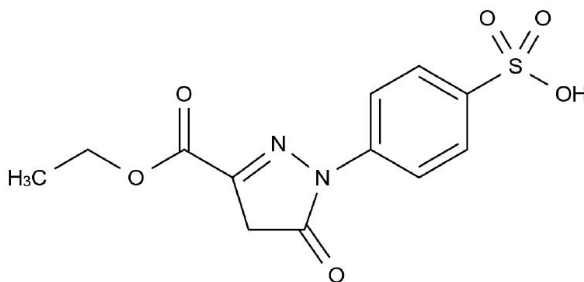
Chemical Structure:
