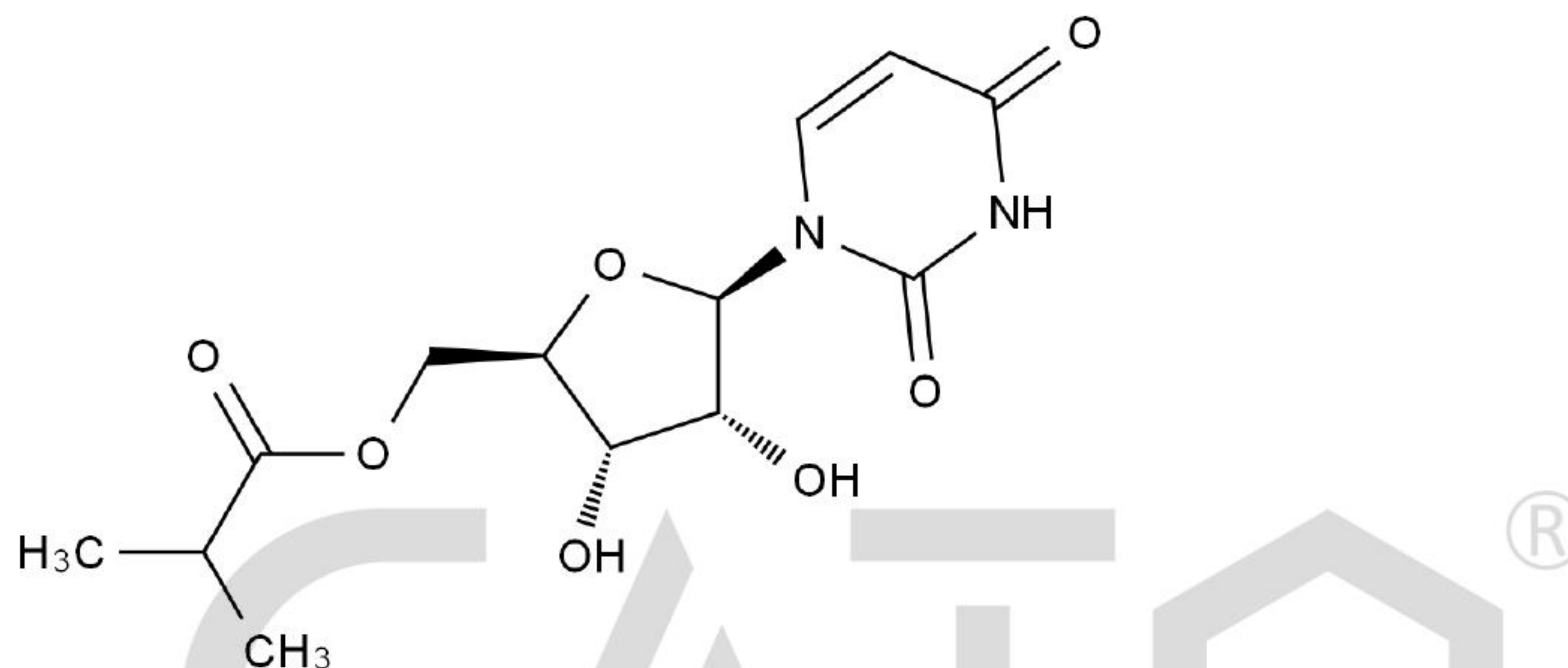
Chemical Structure:
