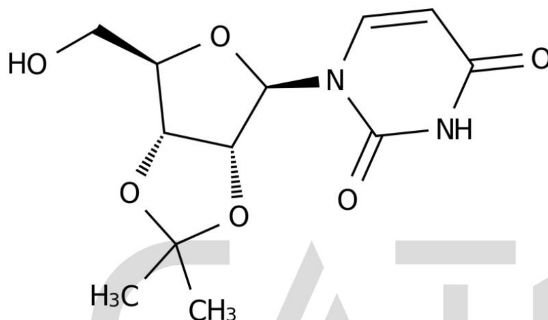
Chemical Structure:
