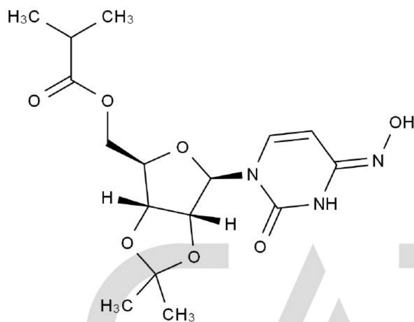
Chemical Structure:
