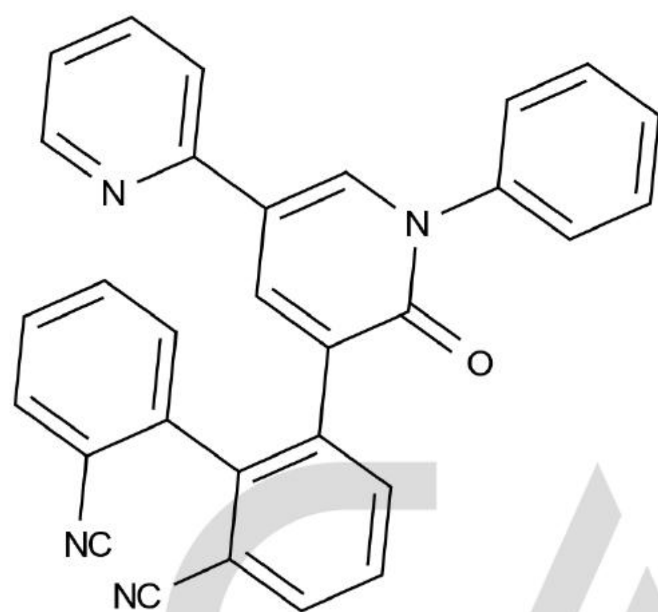
Chemical Structure:
