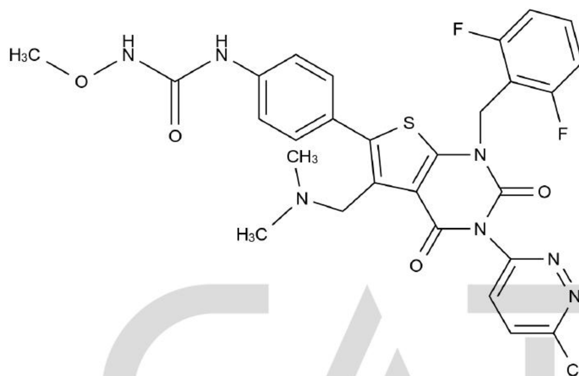
Chemical Structure:
