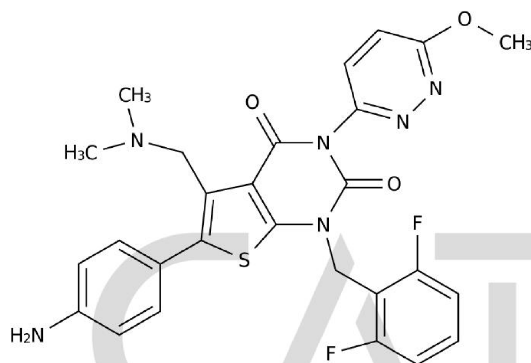
Chemical Structure:
